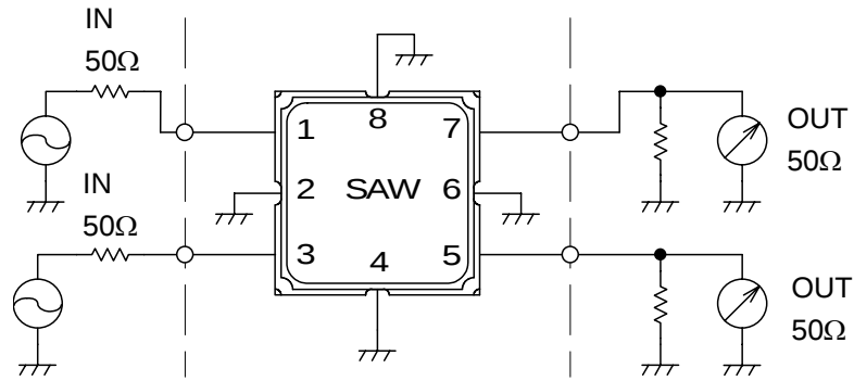
Fig.1 Measuring circuit
